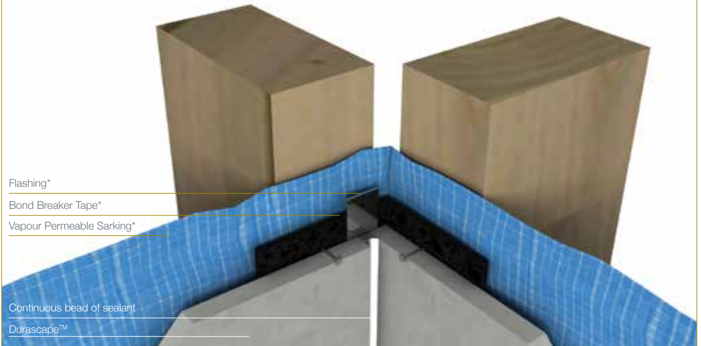
FIGURE 15 INTERNAL CORNER – STEEL
